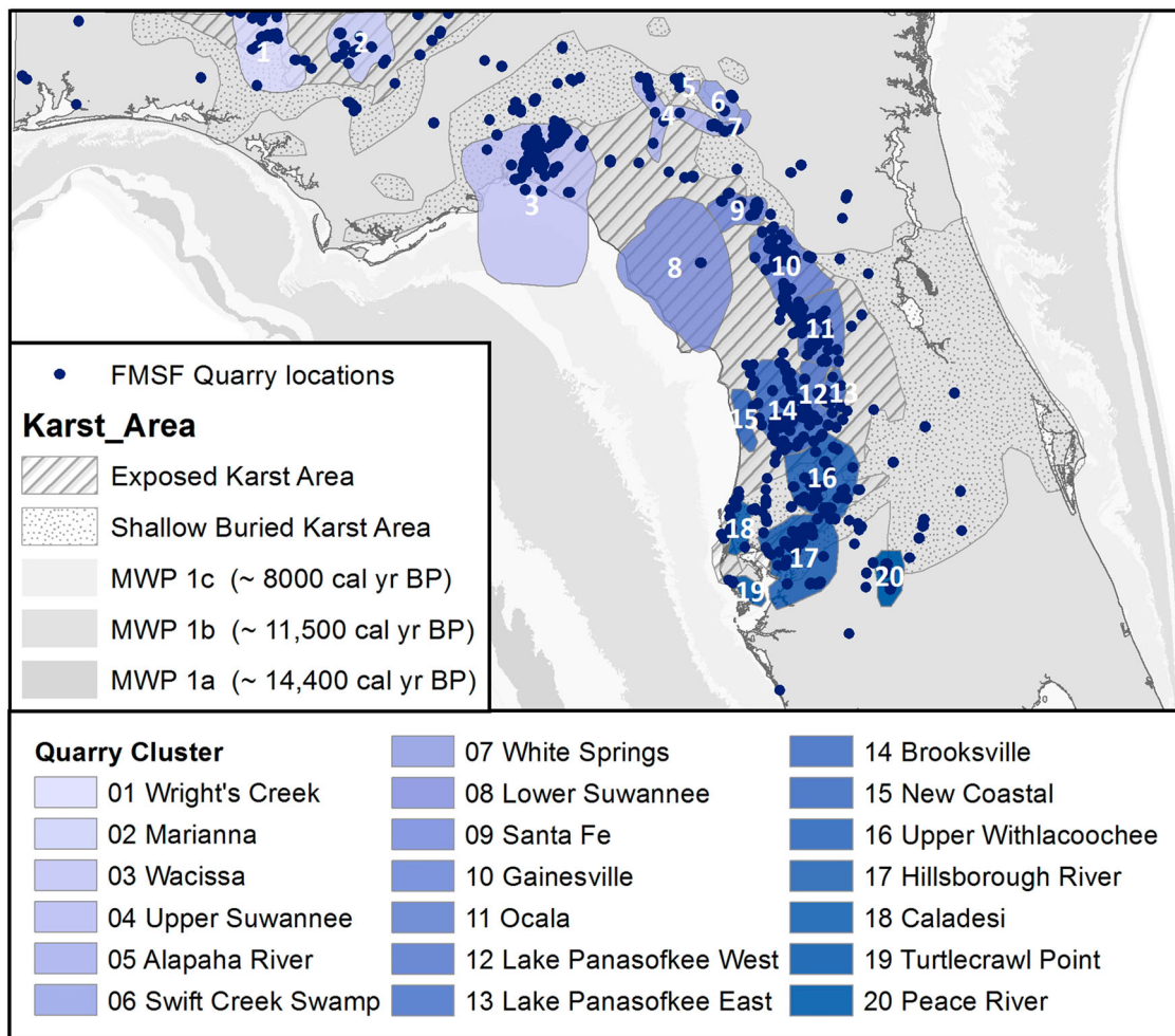
Figure 5 Quarry and quarry cluster locations in Florida (adapted from Austin et al. 2018 and FMSF data). The MWP 1a, 1b, and 1c shelf transgression areas are shown in shades of gray; the timing and extent of the pulses are presented in Table 1. Bathymetric data from NOAA; sea level magnitude and rates from Joy (2018, forthcoming).
